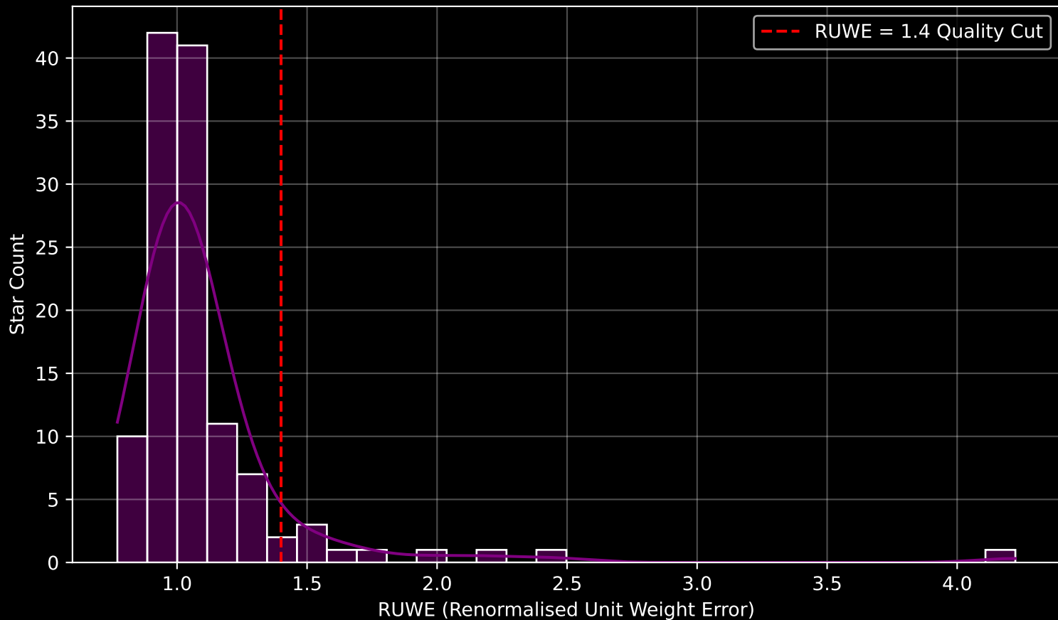
GAPOGEE DR17 Field [022+00] RUWE Distribution (n= 122)
