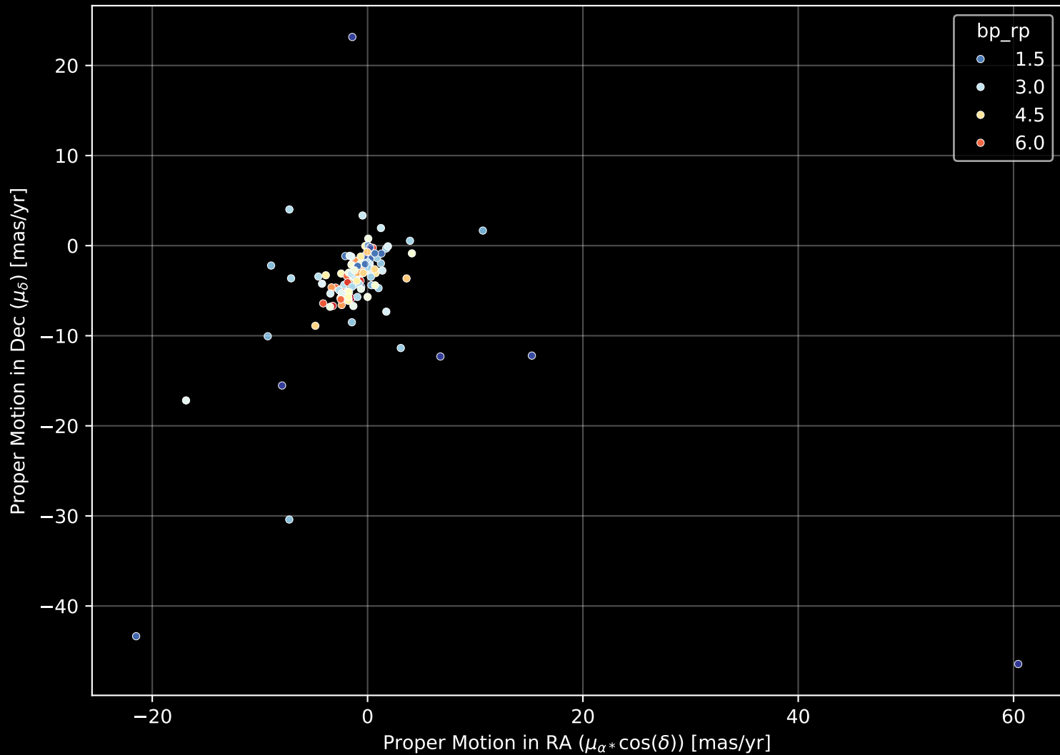
APOGEE DR17 Field: [022+00] Proper Motion Diagram (n= 122)
