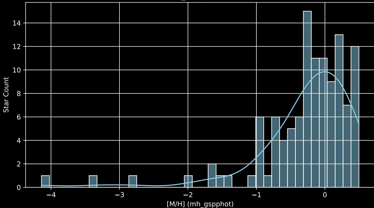
APOGEE DR17 Field: [022+00 [M/H] (mh_gspphot) (n= 115)
