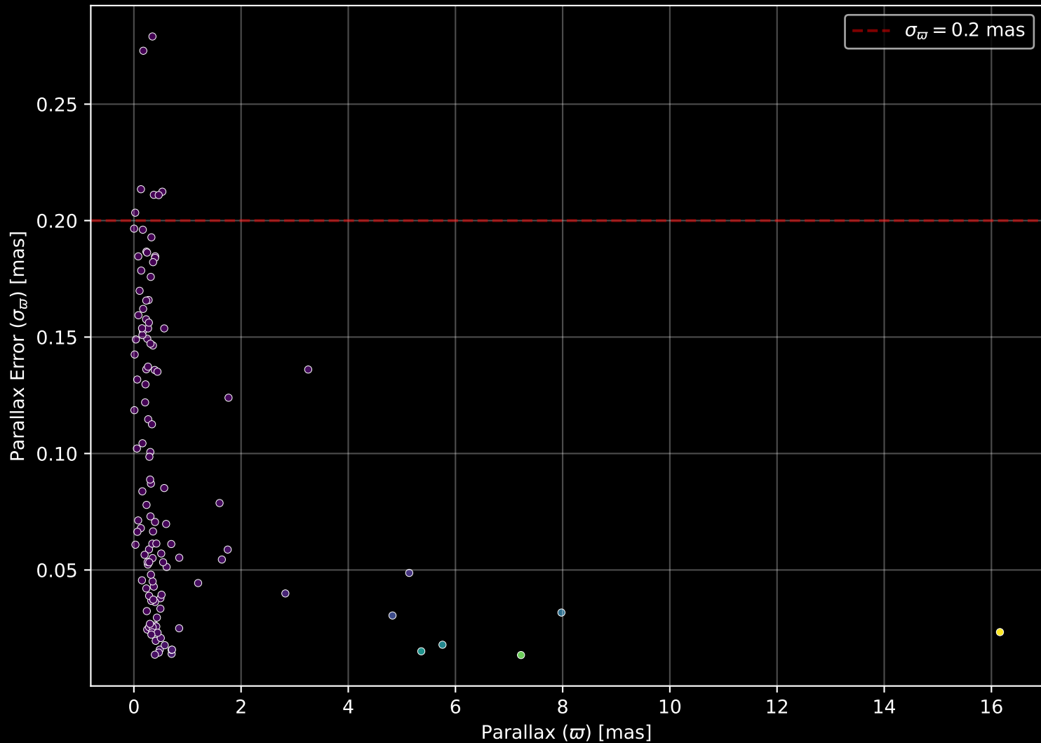
APOGEE DR17 Field: [022+00] Parallax Quality (n= 122)
