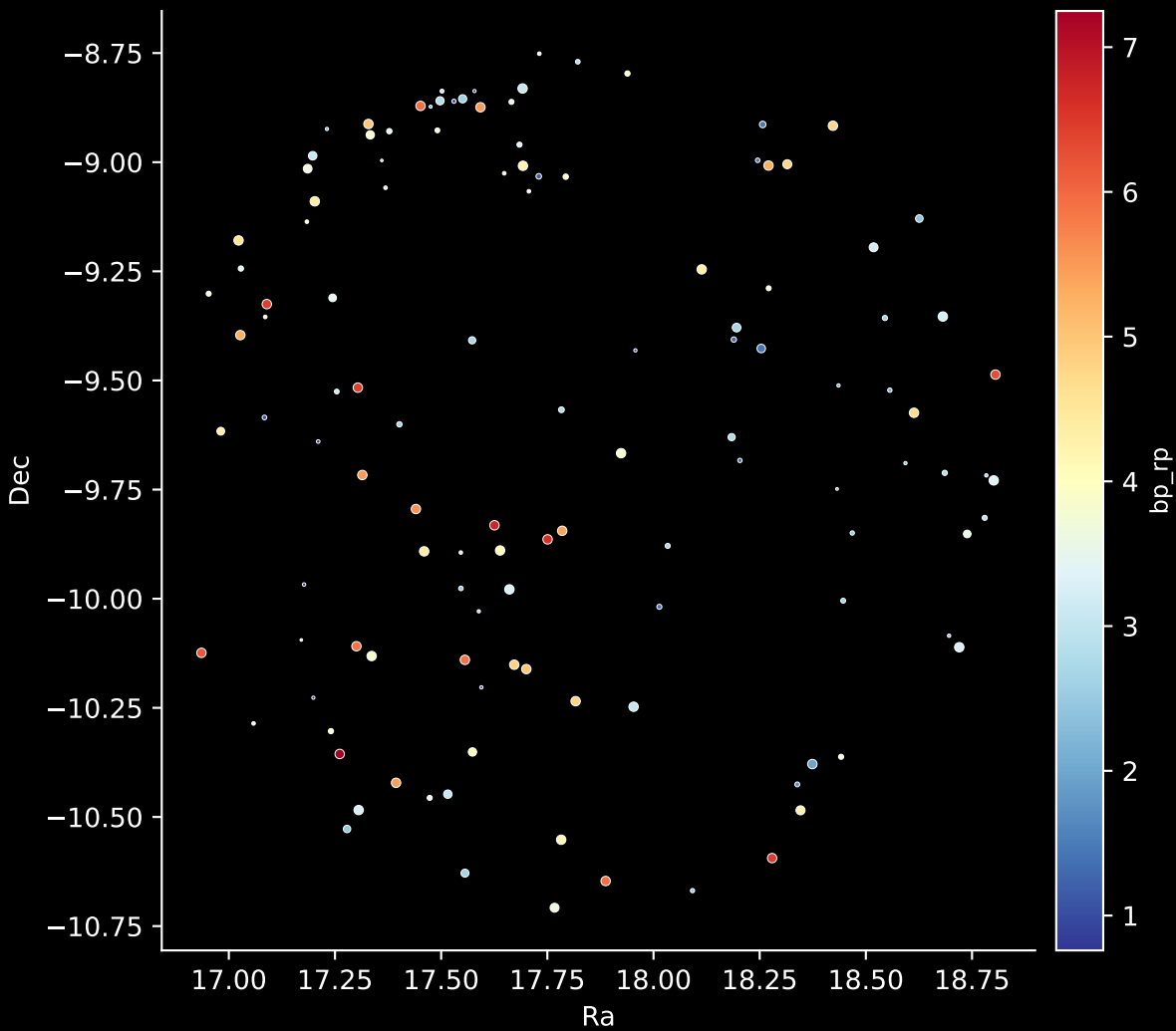
APOGEE DR17 Field: [022+00] Stars: 122
