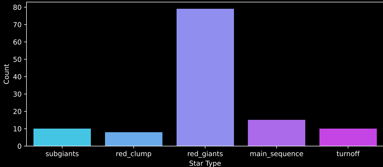
APOGEE DR17 Field: [022+00] Count plot of Star Type
